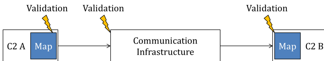
Figure C.1 — Message validation
